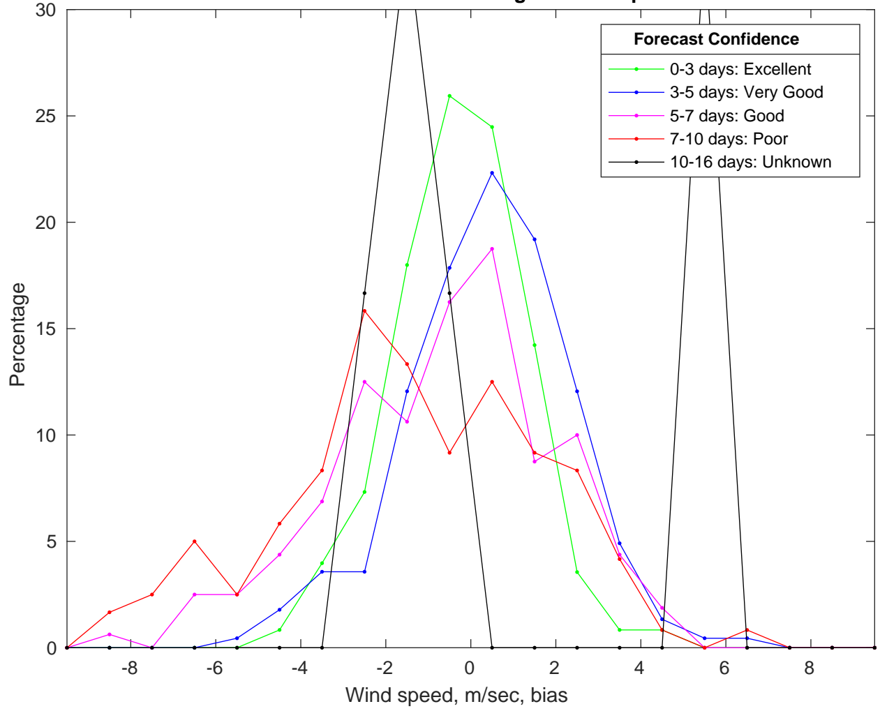
NDBC 46054 vs GFS Winds Bias Histogram: 19-Sep-2024
