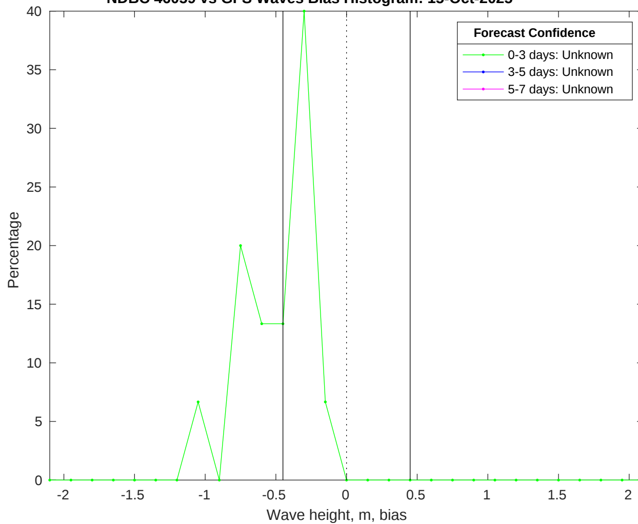
NDBC 46059 vs GFS Waves Bias Histogram: 15-Oct-2025
