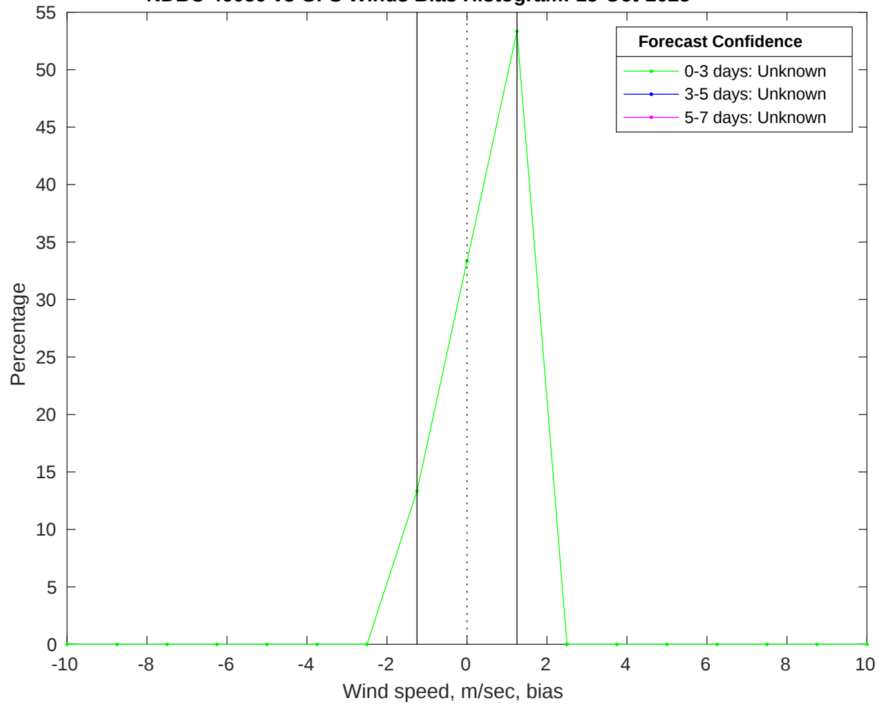
NDBC 46059 vs GFS Winds Bias Histogram: 15-Oct-2025
