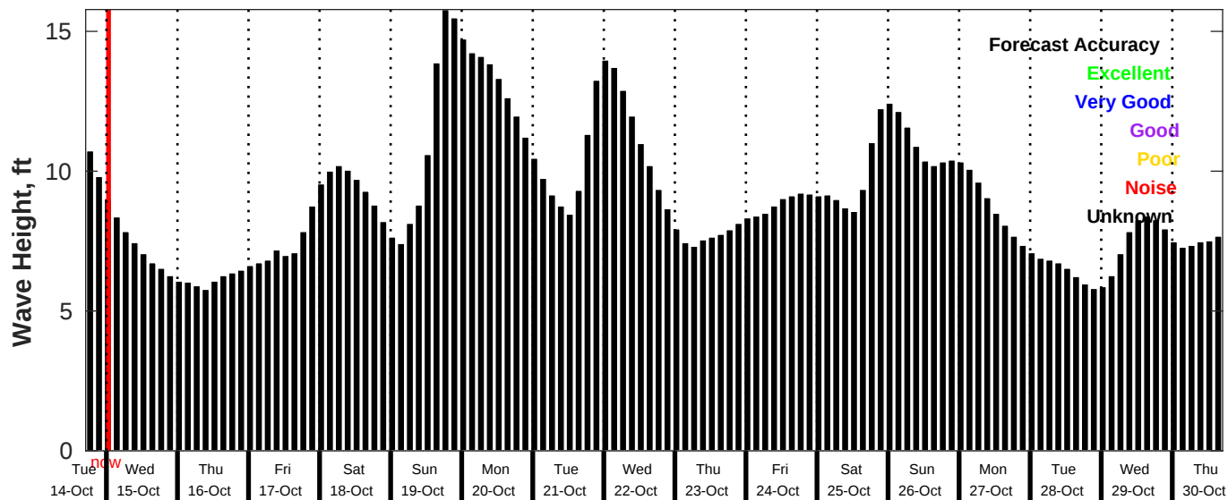
GFS Wave Forecast for NDBC 46059 from 14-Oct-2025 17:00:00 to 30-Oct-2025 17:00:00
