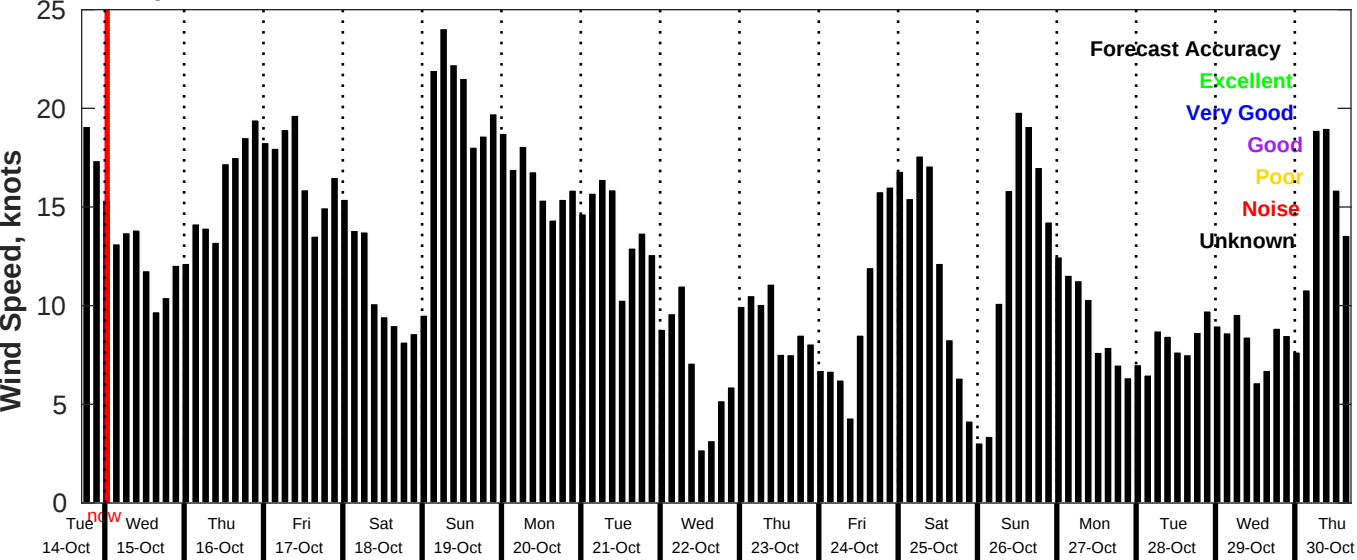
GFS Wind Speed Forecast for NDBC 46059 from 14-Oct-2025 17:00:00 to 30-Oct-2025 17:00:00
