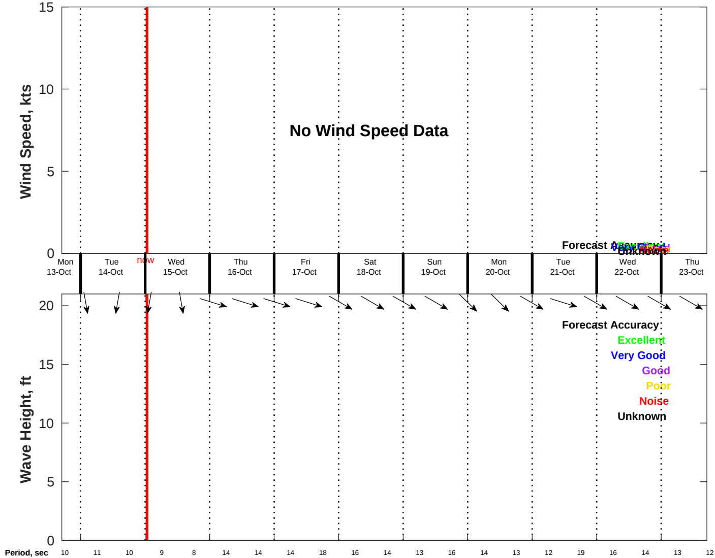
Wind & Wave Forecast for NDBC 46059 from 13-Oct-2025 17:00:00 to 23-Oct-2025 17:00:00
