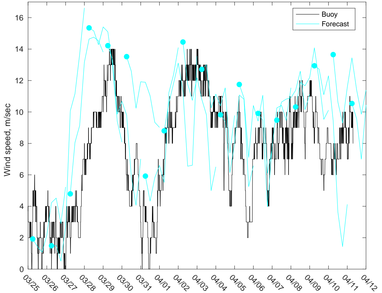
NDBC 46069 vs AUSWAV Winds: 5 to 7 day forecast
