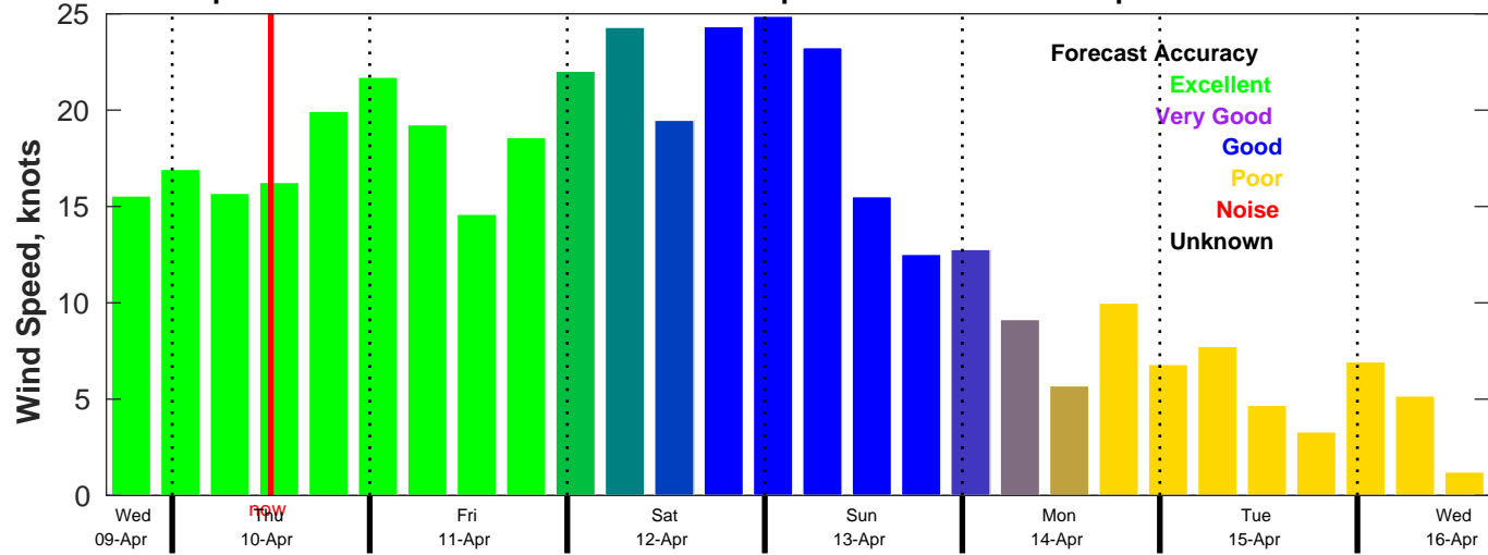
AUSWAV Wind Speed Forecast for NDBC 46069 from 09-Apr-2025 16:00:00 to 16-Apr-2025 16:00:00
