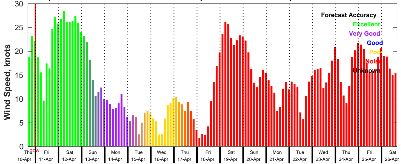
GFS Wind Speed Forecast for NDBC 46069 from 10-Apr-2025 16:00:00 to 26-Apr-2025 16:00:00
