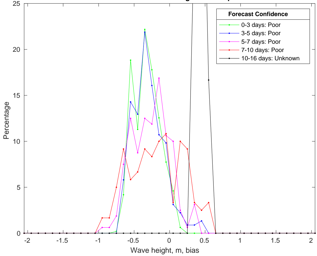
NDBC 46069 vs GFSWaves Bias Histogram: 19-Sep-2024
