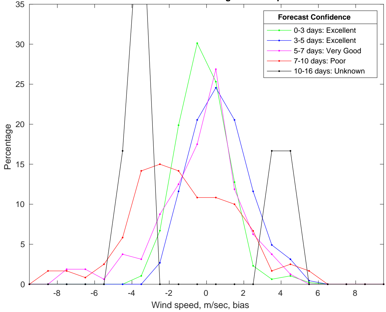
NDBC 46069 vs GFS Winds Bias Histogram: 19-Sep-2024
