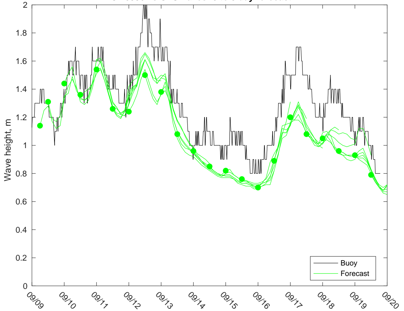
NDBC 46086 vs GFSWaves: 0 to 3 day forecast
