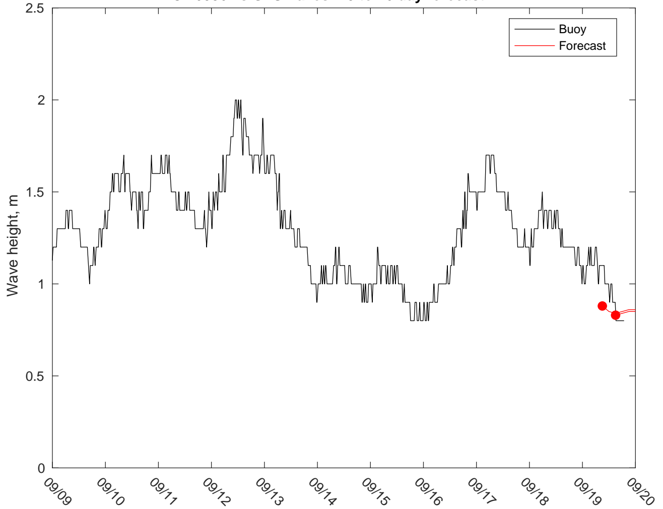
NDBC 46086 vs GFSWaves: 10 to 16 day forecast
