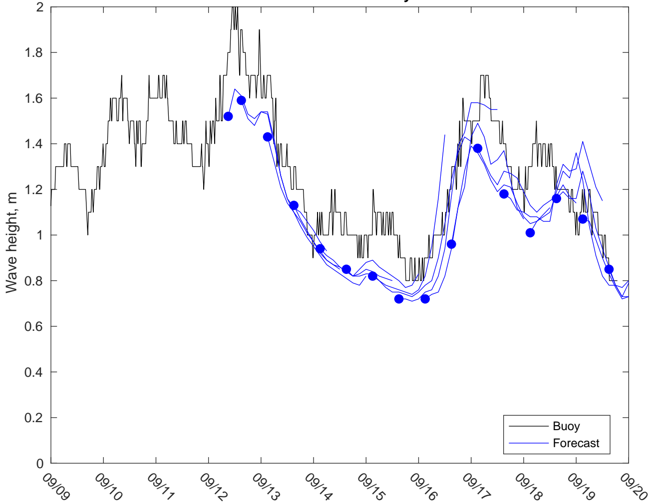
NDBC 46086 vs GFSWaves: 3 to 5 day forecast
