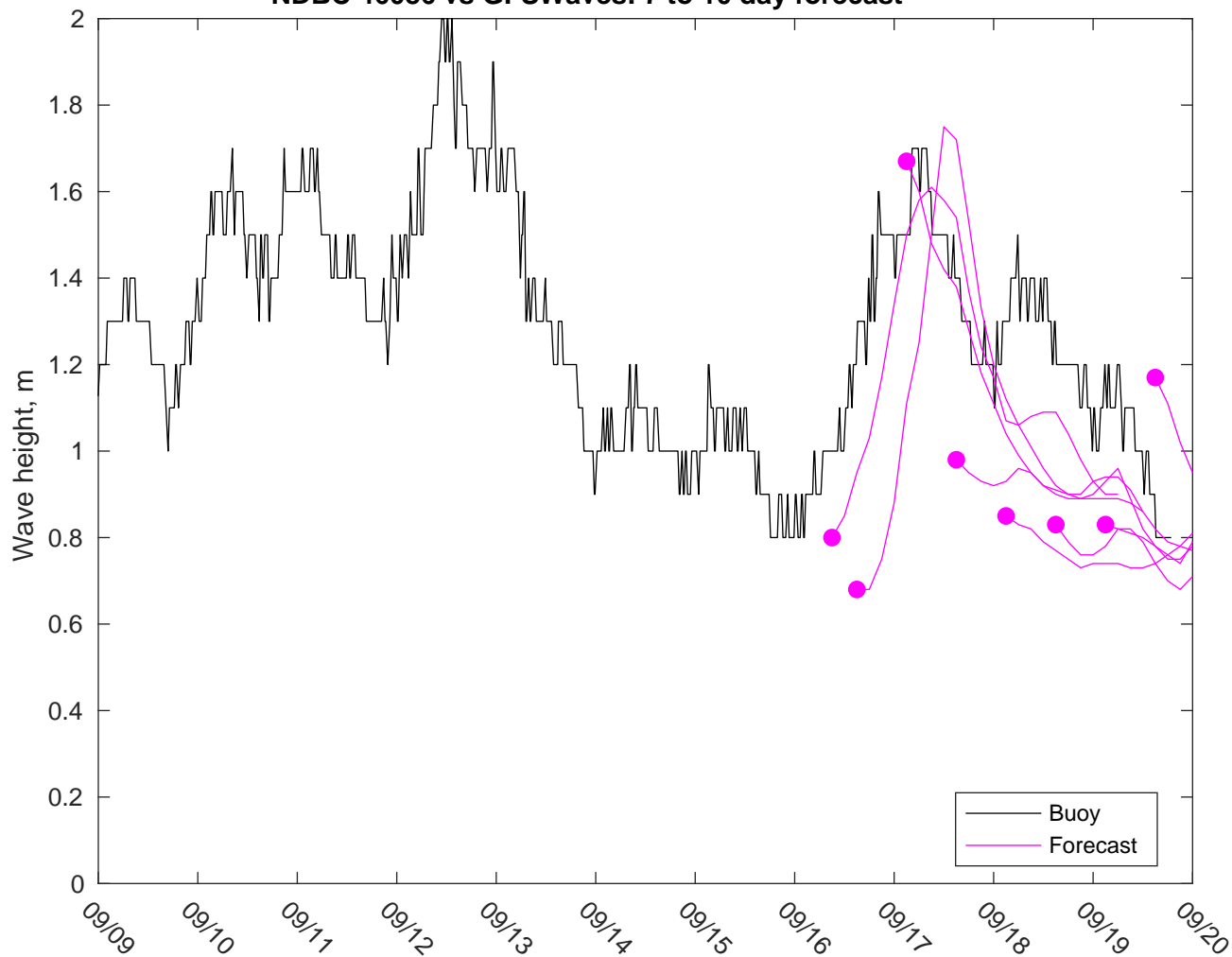
NDBC 46086 vs GFSWaves: 7 to 10 day forecast
