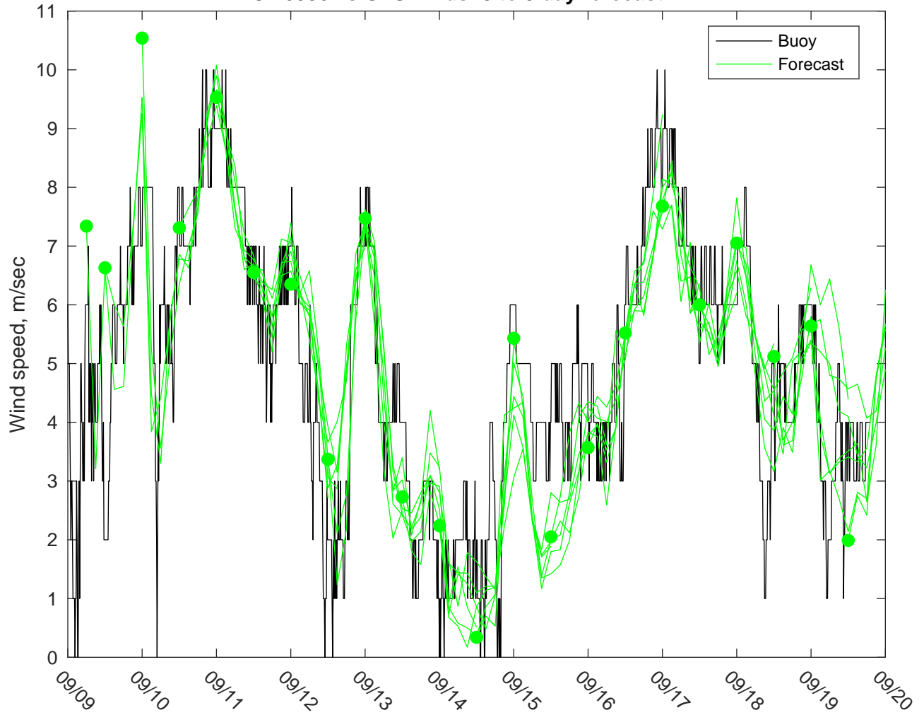
NDBC 46086 vs GFSWinds: 0 to 3 day forecast
