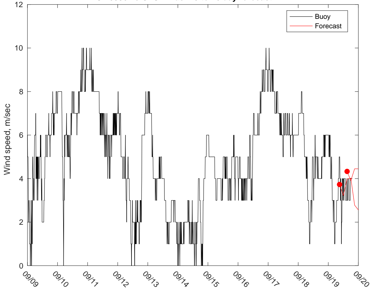
NDBC 46086 vs GFSWinds: 10 to 16 day forecast
