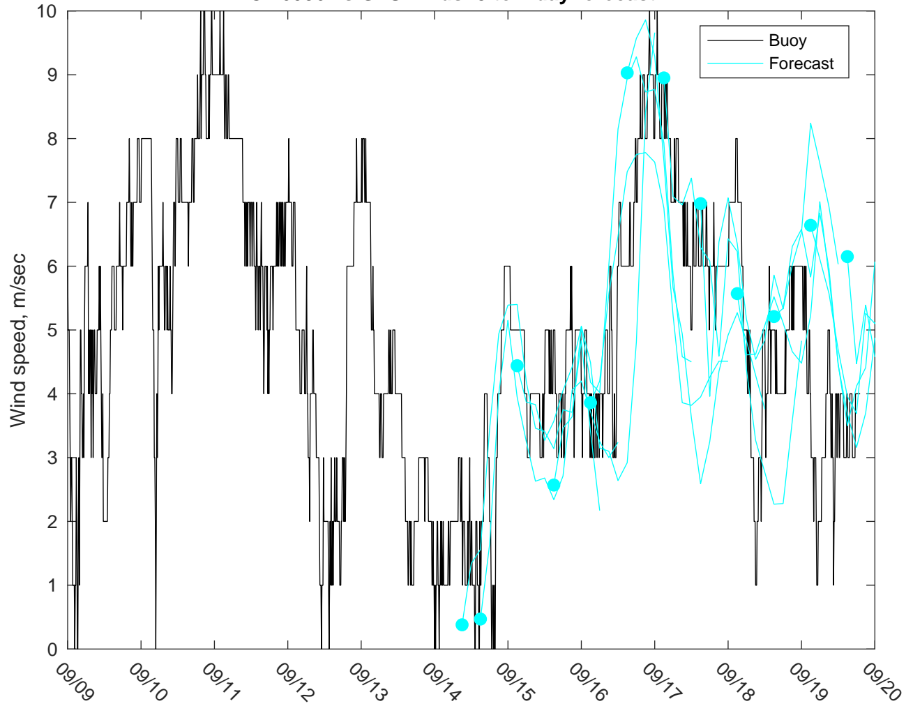
NDBC 46086 vs GFSWinds: 5 to 7 day forecast
