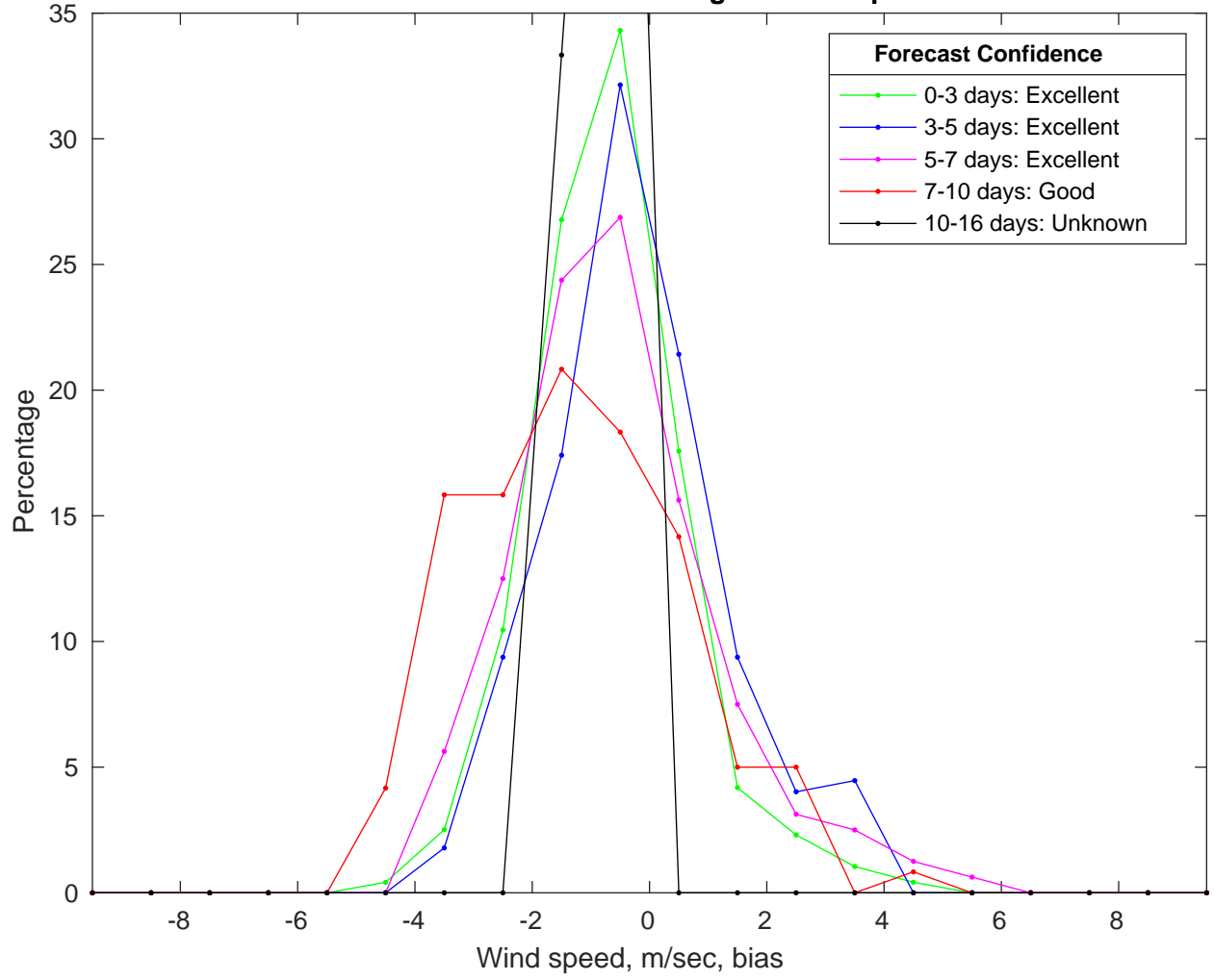
NDBC 46086 vs GFS Winds Bias Histogram: 19-Sep-2024
