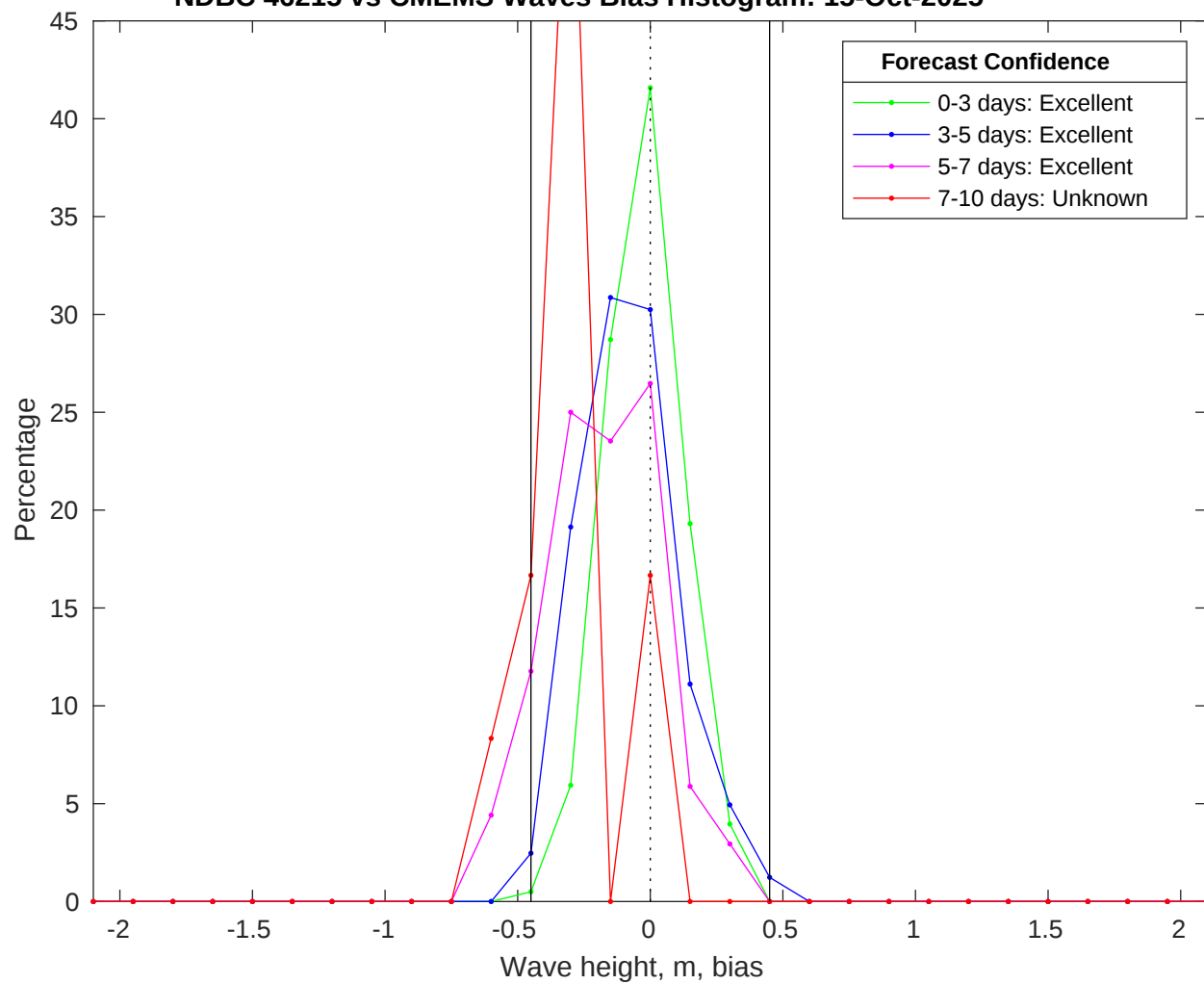
NDBC 46215 vs CMEMS Waves Bias Histogram: 15-Oct-2025
