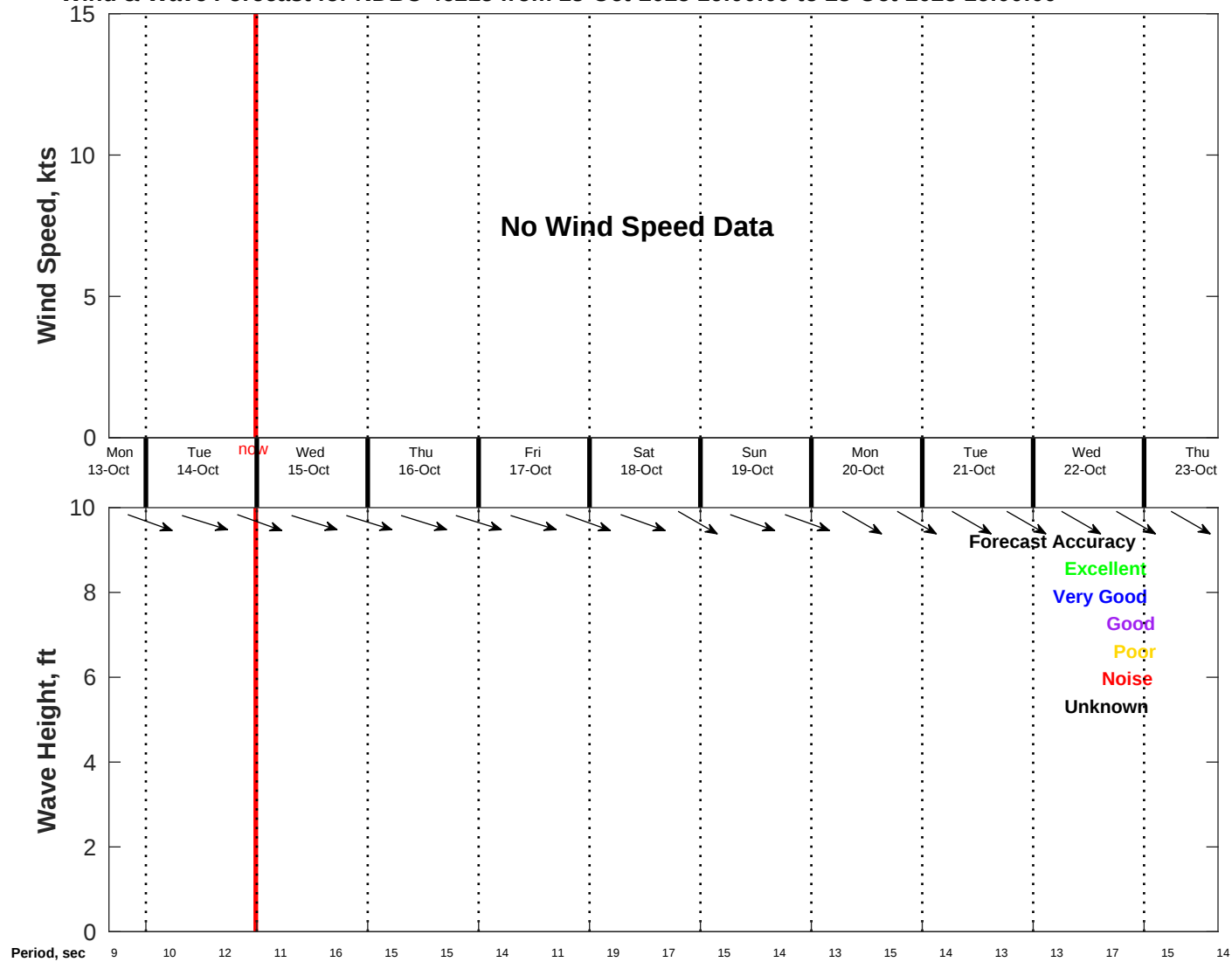
Wind & Wave Forecast for NDBC 46215 from 13-Oct-2025 16:00:00 to 23-Oct-2025 16:00:00
