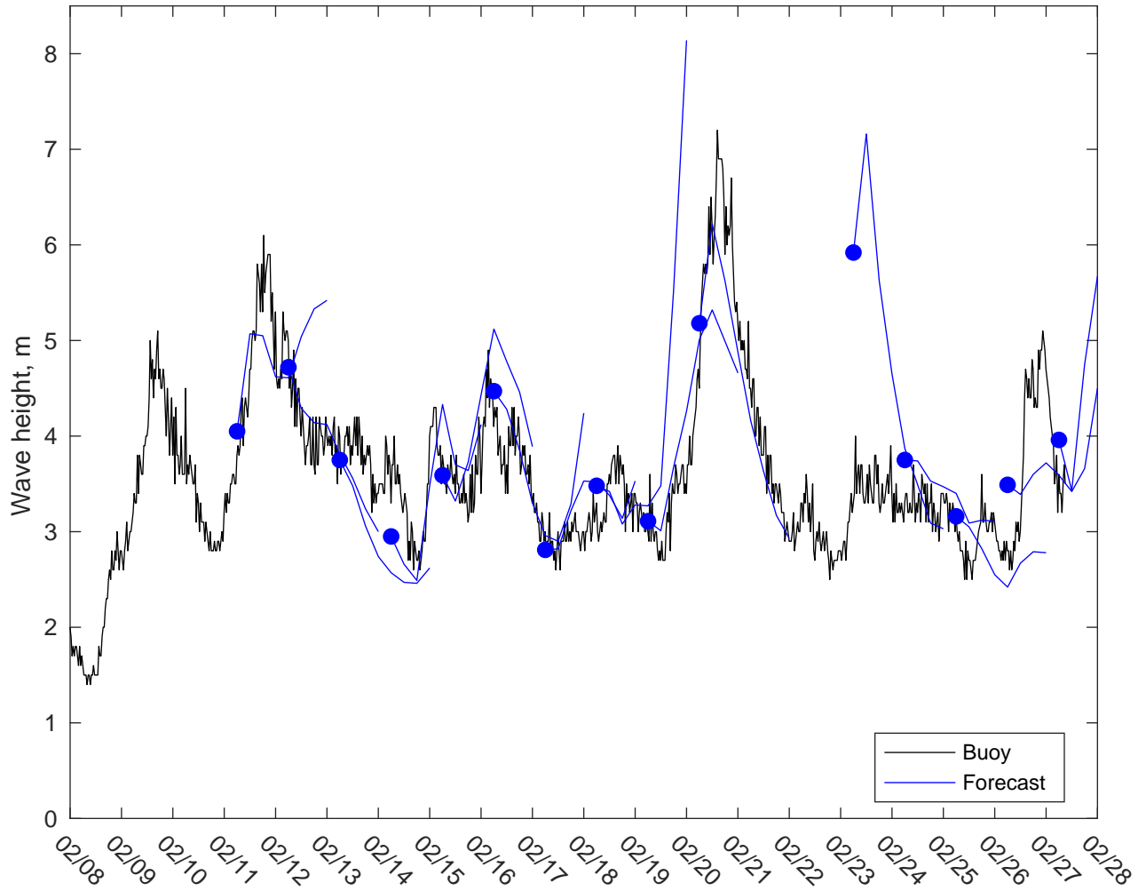
NDBC 46246 vs AUSWAV Waves: 3 to 5 day forecast
