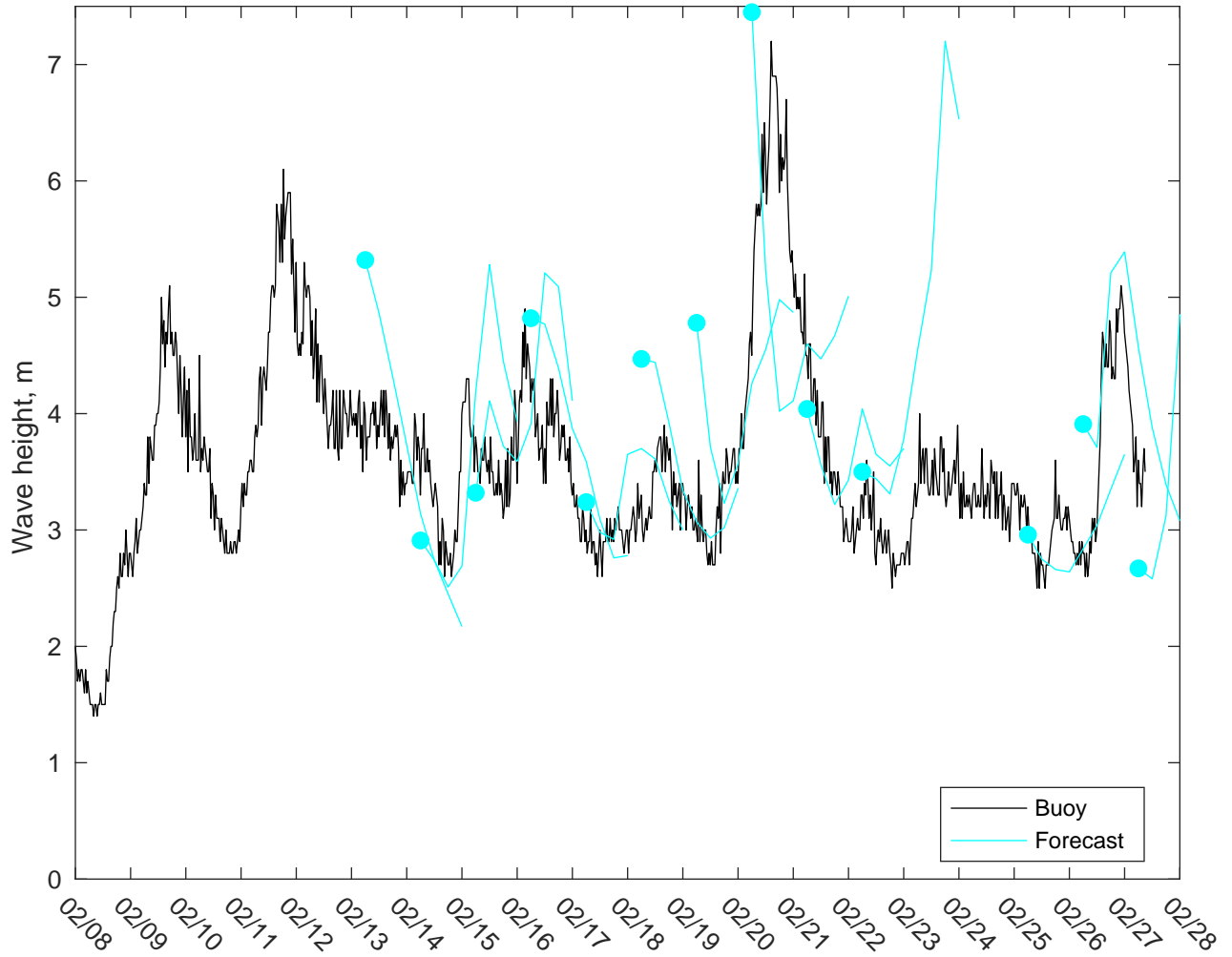
NDBC 46246 vs AUSWAV Waves: 5 to 7 day forecast
