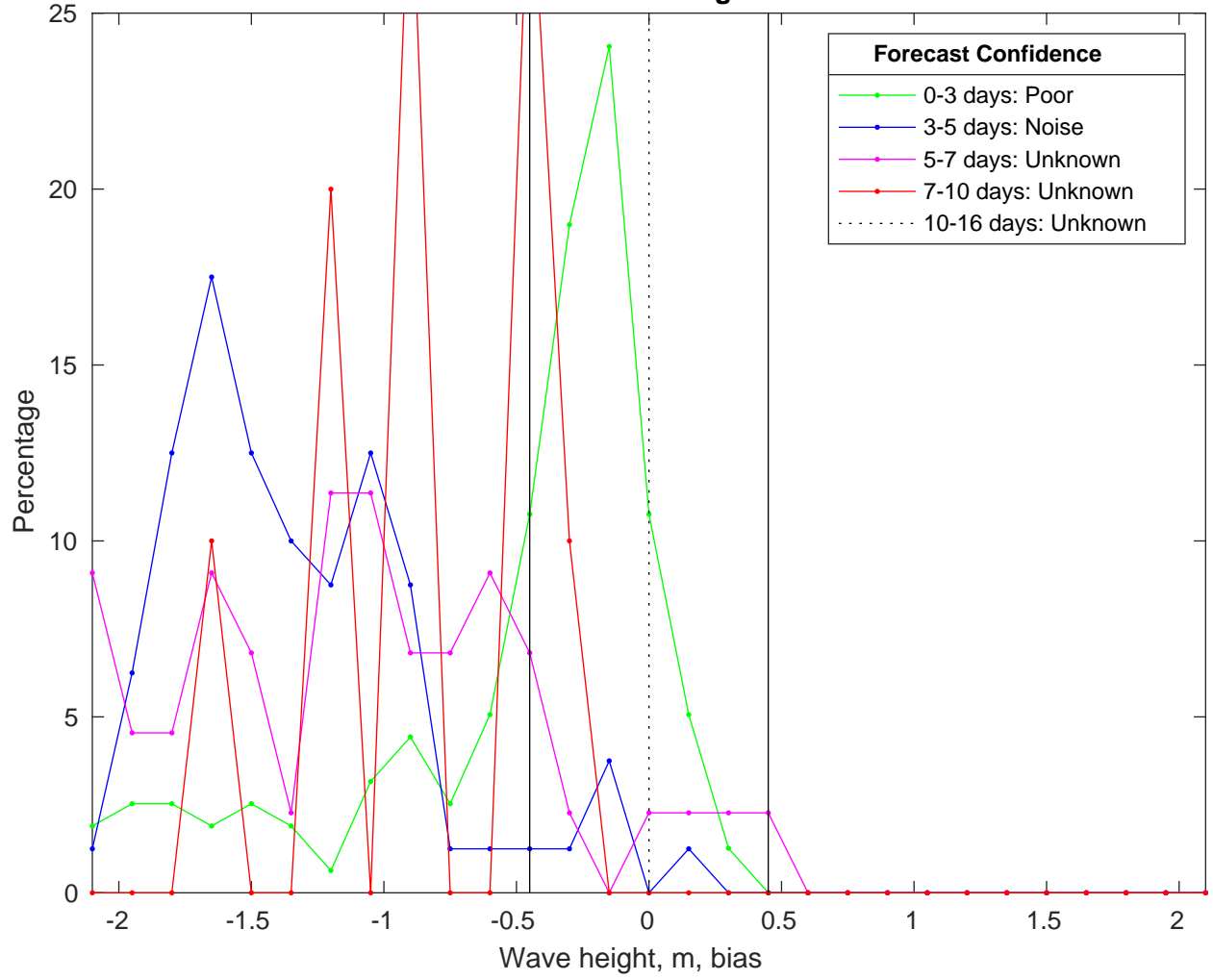
NDBC 46246 vs GFSWaves Bias Histogram: 18-Jan-2025
