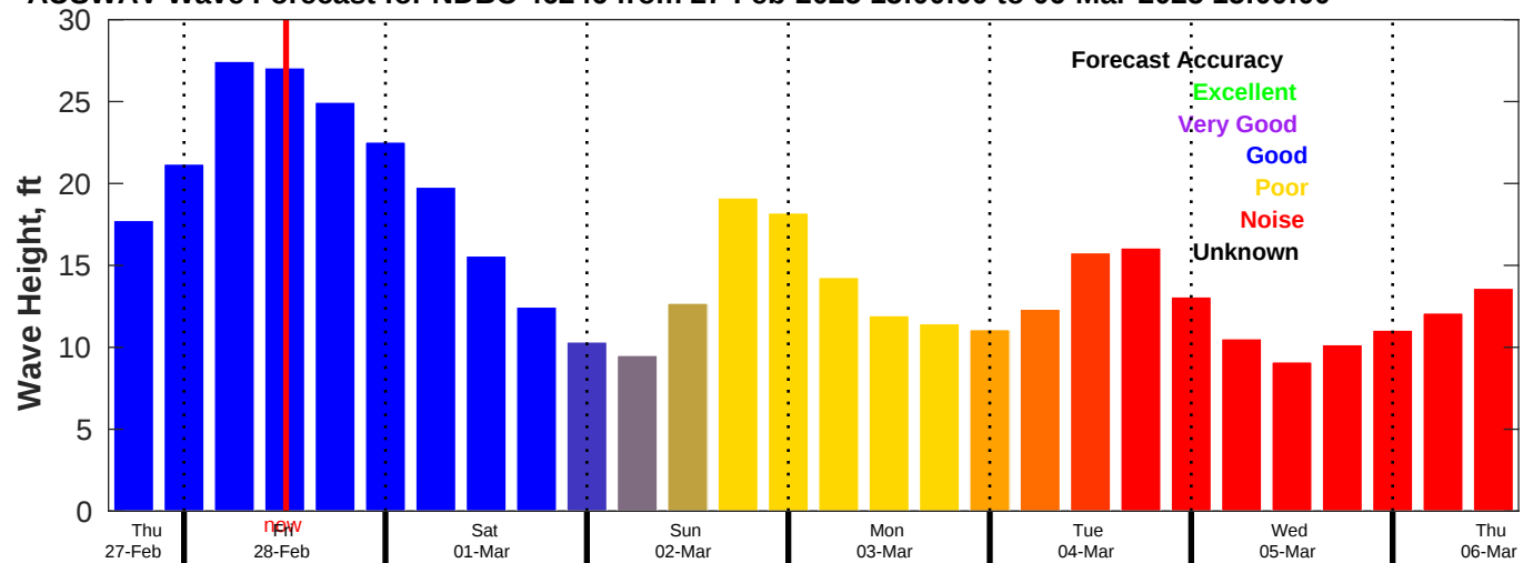
AUSWAV Wave Forecast for NDBC 46246 from 27-Feb-2025 15:00:00 to 06-Mar-2025 15:00:00
