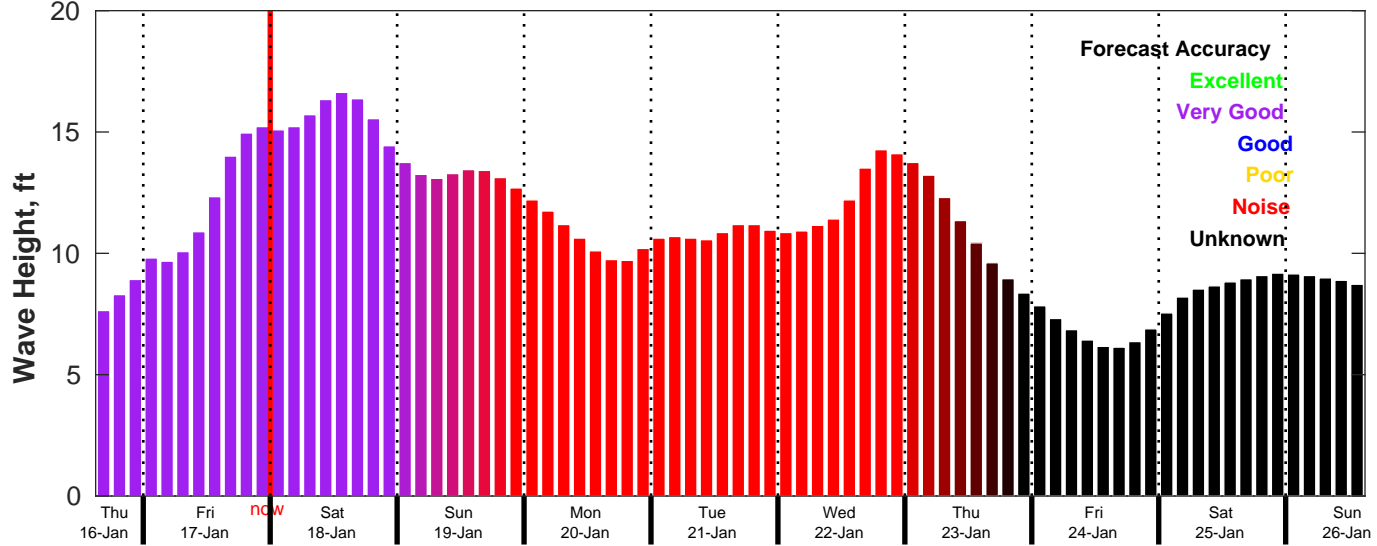
CMEMS Wave Forecast for NDBC 46246 from 16-Jan-2025 15:00:00 to 26-Jan-2025 15:00:00
