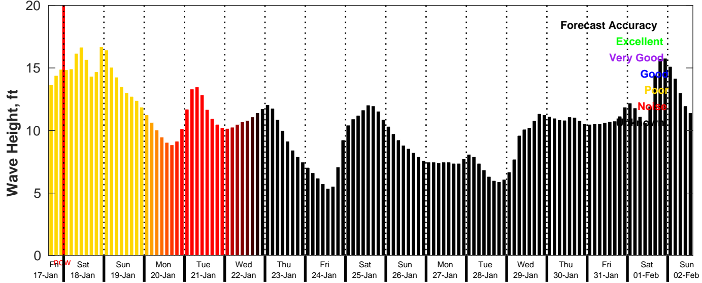
GFS Wave Forecast for NDBC 46246 from 17-Jan-2025 15:00:00 to 02-Feb-2025 15:00:00
