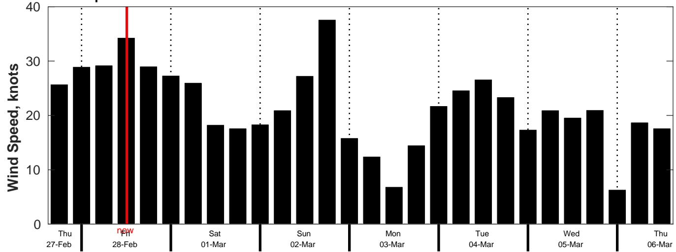
AUSWAV Wind Speed Forecast for NDBC 46246 from 27-Feb-2025 15:00:00 to 06-Mar-2025 15:00:00
