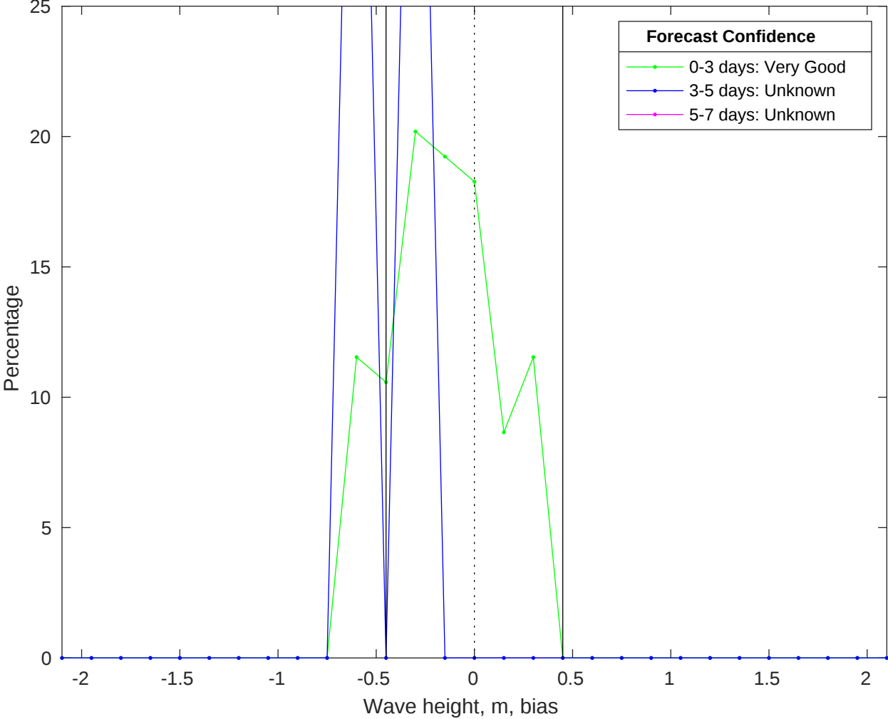
NDBC 46259 vs CMEMS Waves Bias Histogram: 15-Oct-2025
