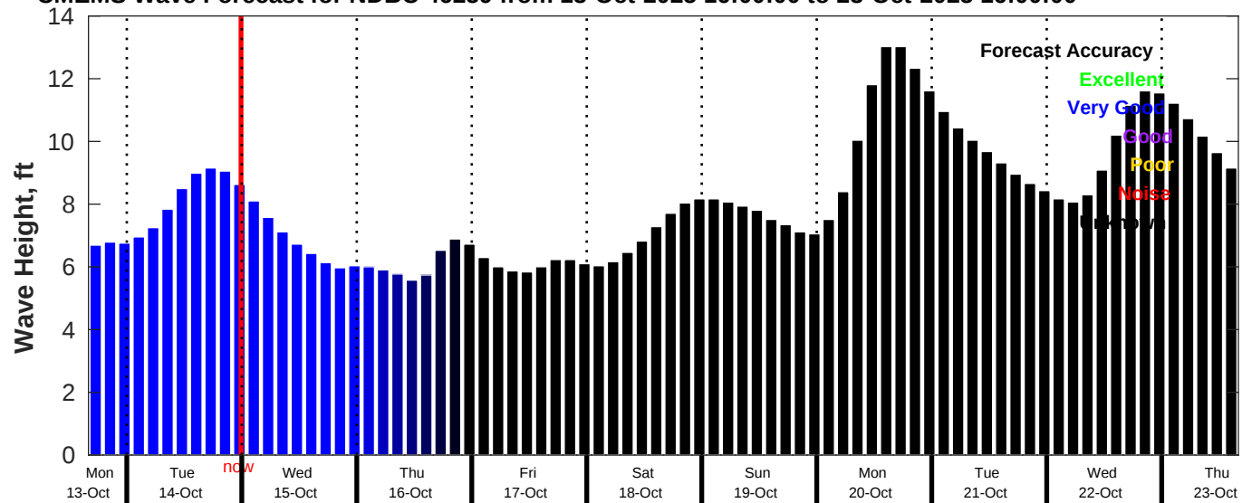
CMEMS Wave Forecast for NDBC 46259 from 13-Oct-2025 16:00:00 to 23-Oct-2025 16:00:00
