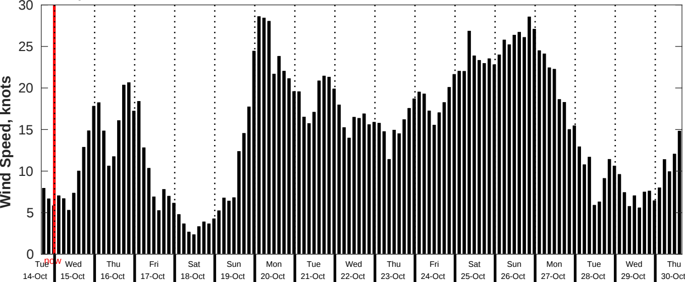
GFS Wind Speed Forecast for NDBC 46259 from 14-Oct-2025 16:00:00 to 30-Oct-2025 16:00:00
