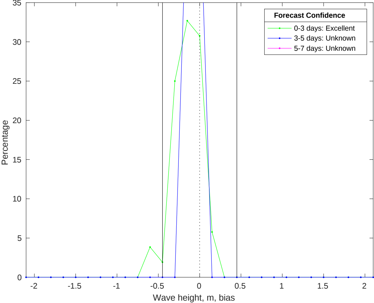
NDBC 51000 vs CMEMS Waves Bias Histogram: 15-Oct-2025
