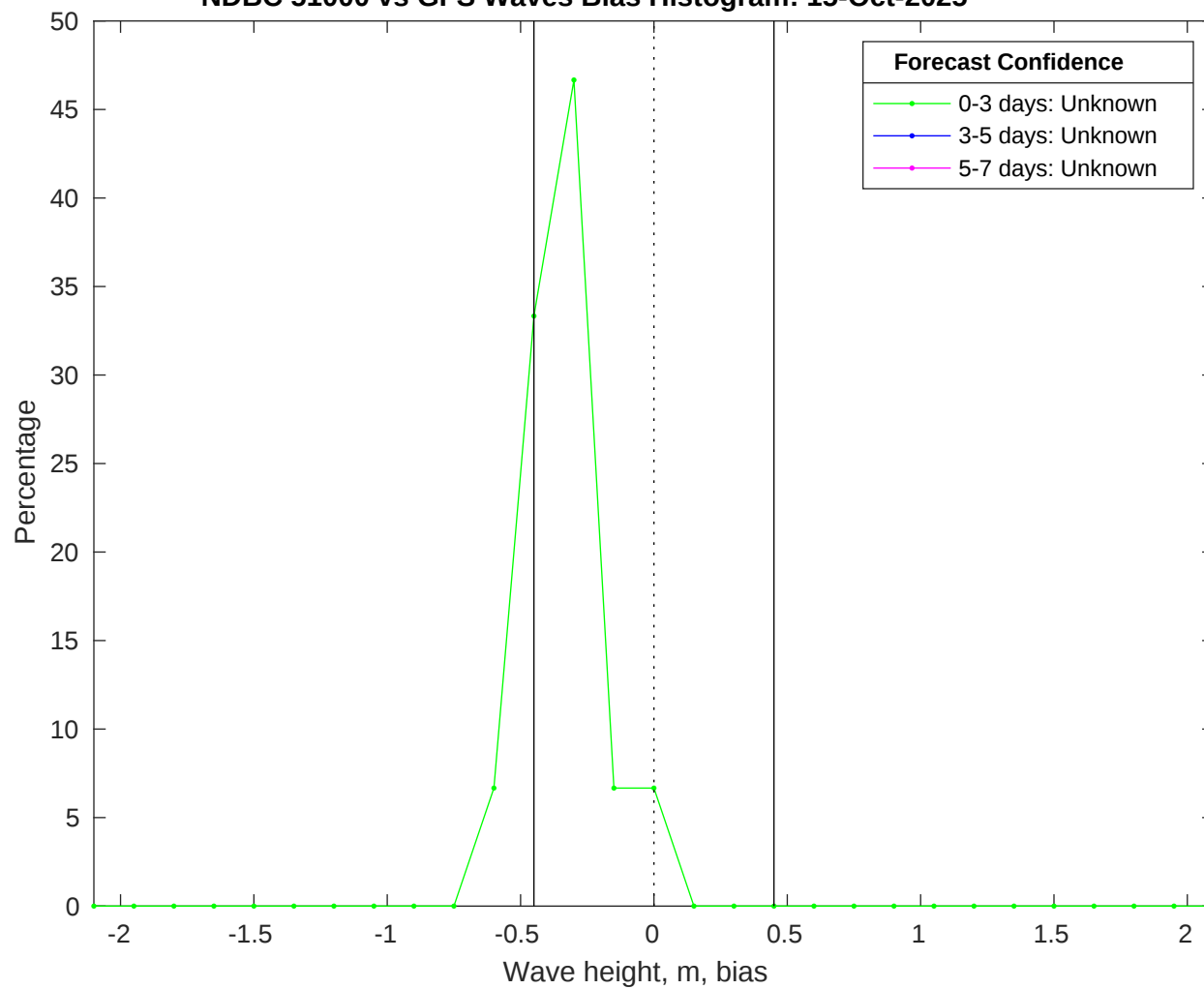
NDBC 51000 vs GFS Waves Bias Histogram: 15-Oct-2025
