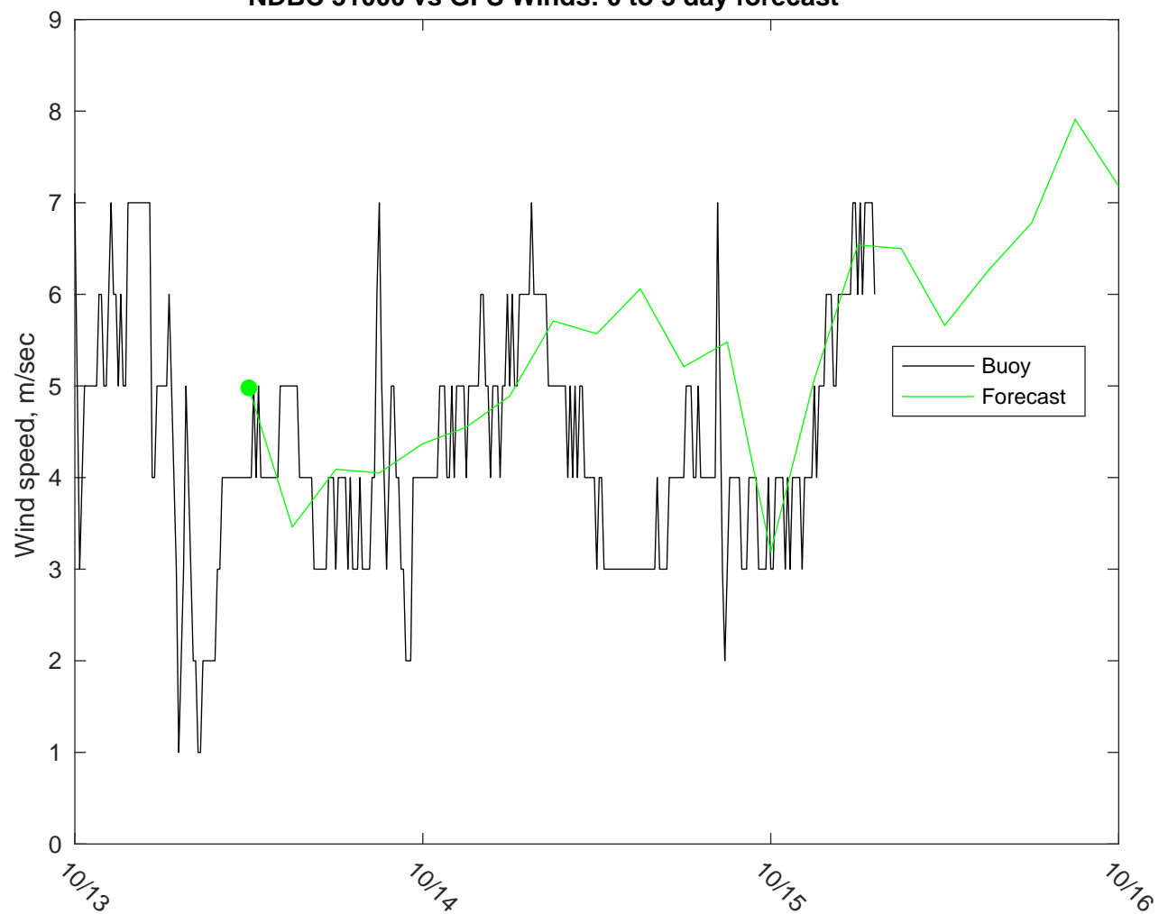
NDBC 51000 vs GFS Winds: 0 to 3 day forecast
