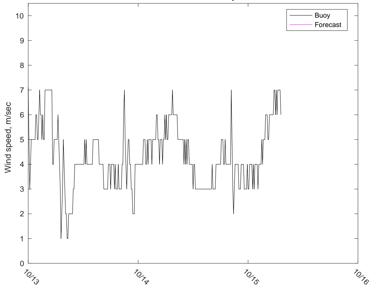
NDBC 51000 vs GFS Winds: 7 to 10 day forecast
