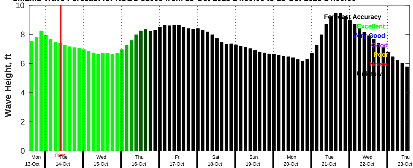
CMEMS Wave Forecast for NDBC 51000 from 13-Oct-2025 14:00:00 to 23-Oct-2025 14:00:00
