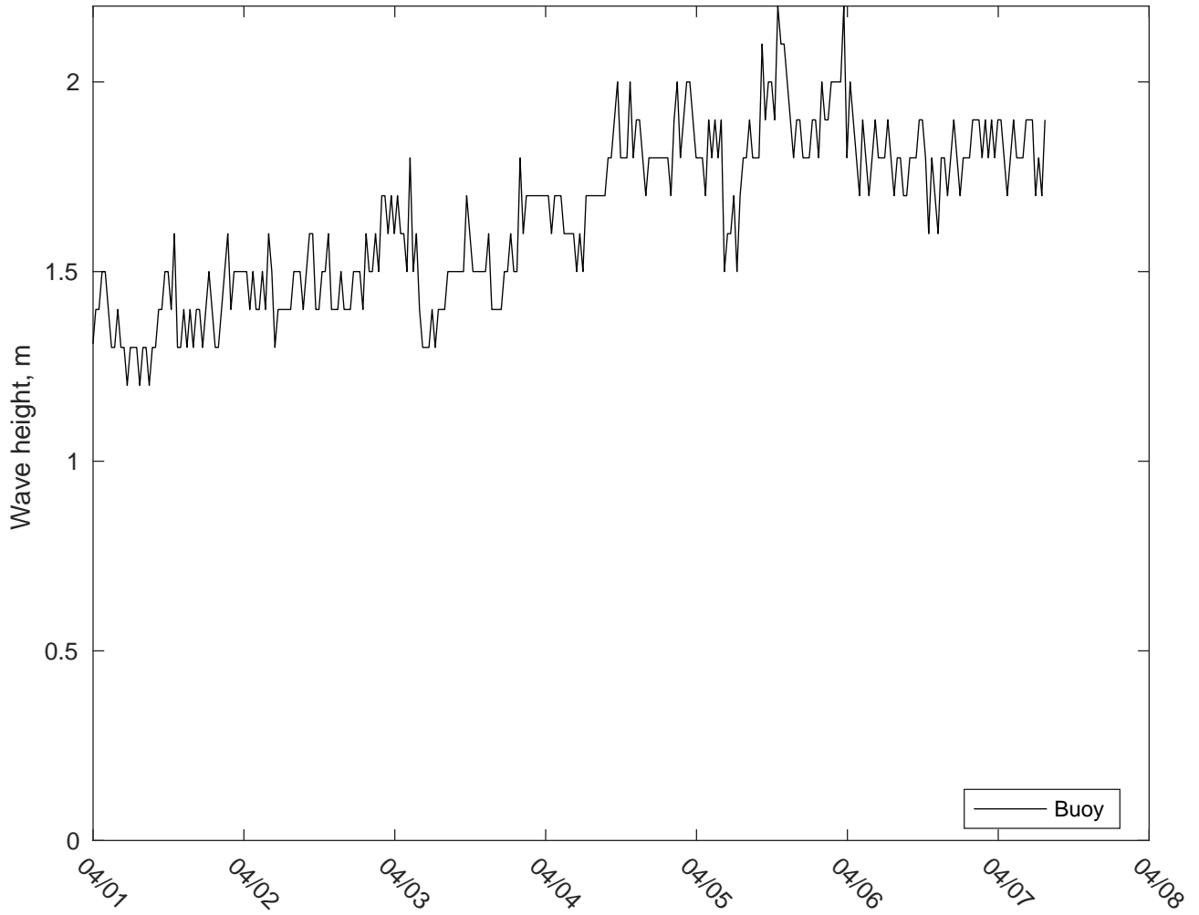
NDBC 51209 vs AUSWAV Waves: 10 to 16 day forecast
