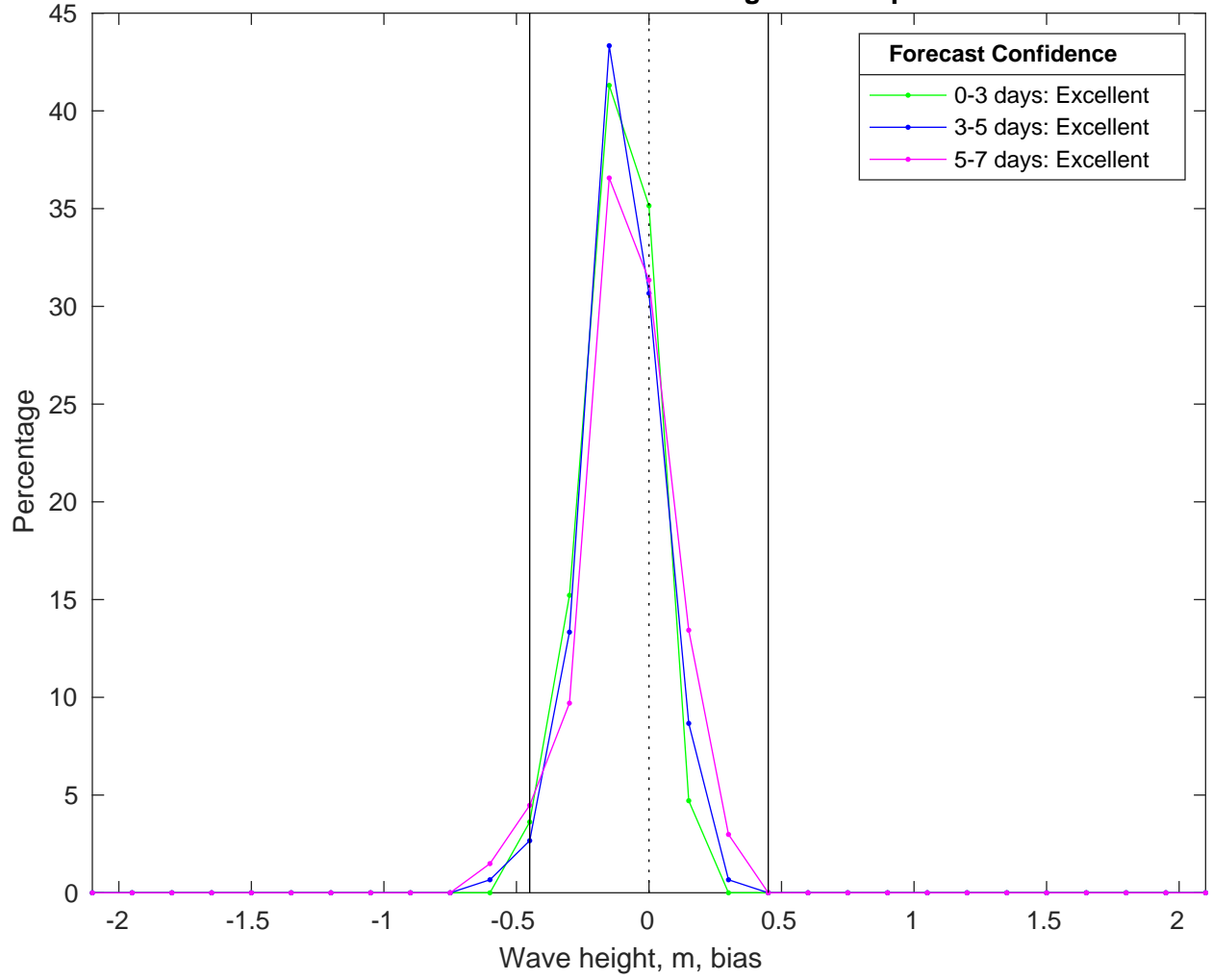
NDBC 51209 vs AUSWAV Waves Bias Histogram: 07-Apr-2025
