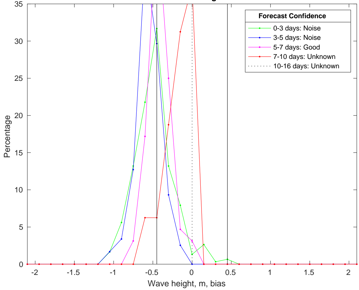
NDBC 51209 vs GFSWaves Bias Histogram: 18-Jan-2025
