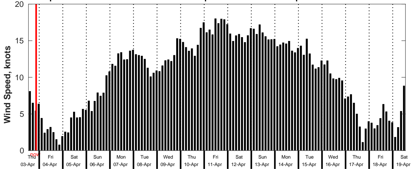
GFS Wind Speed Forecast for NDBC 51209 from 03-Apr-2025 13:00:00 to 19-Apr-2025 13:00:00
