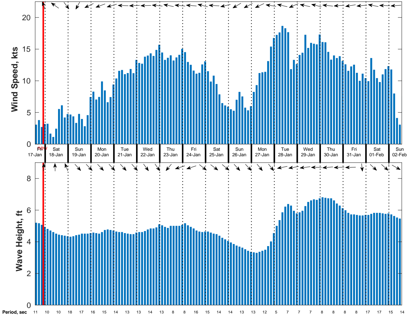
Wind & Wave Forecast for NDBC 51209 from 17-Jan-2025 13:00:00 to 02-Feb-2025 13:00:00
