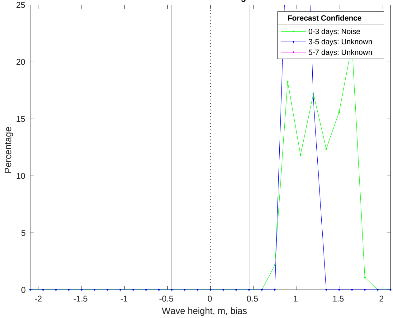
NDBC 51211 vs CMEMS Waves Bias Histogram: 16-Jul-2025
