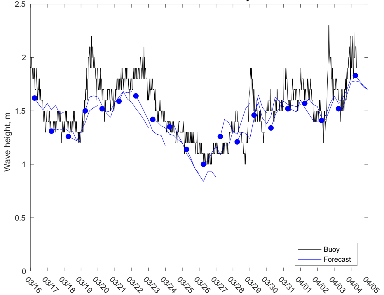
NDBC 52211 vs AUSWAV Waves: 3 to 5 day forecast
