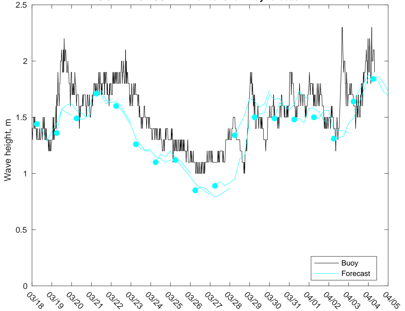
NDBC 52211 vs AUSWAV Waves: 5 to 7 day forecast
