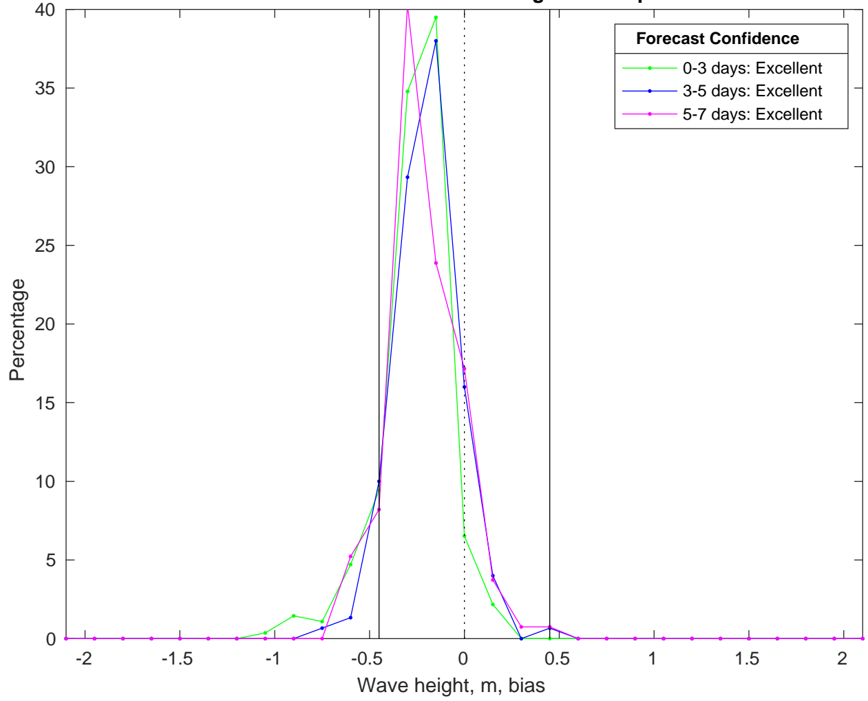
NDBC 52211 vs AUSWAV Waves Bias Histogram: 04-Apr-2025
