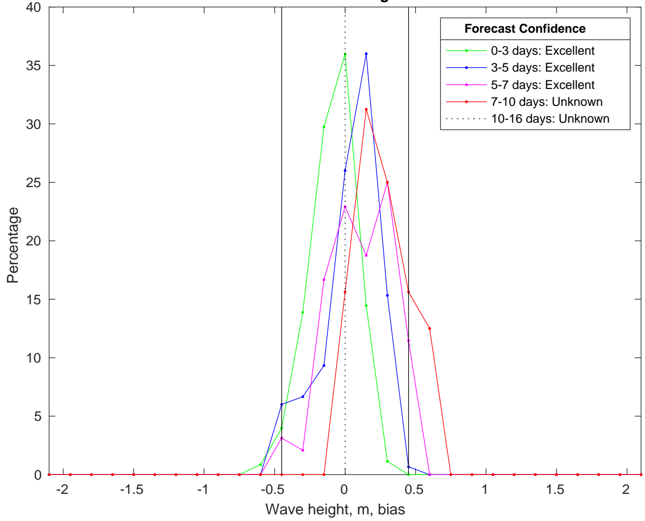
NDBC 52211 vs GFSWaves Bias Histogram: 18-Jan-2025
