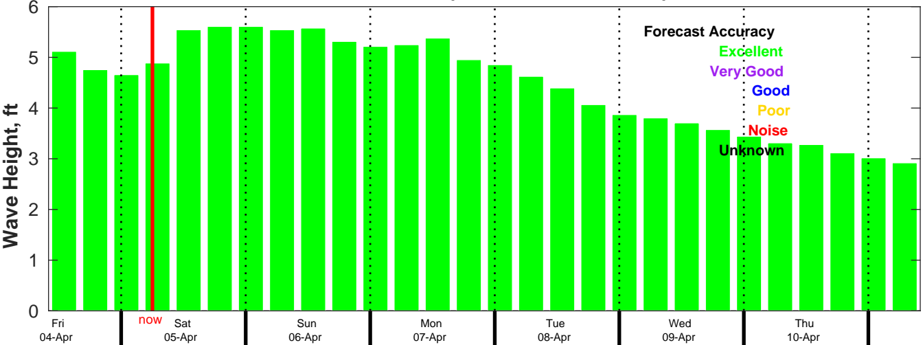
AUSWAV Wave Forecast for NDBC 52211 from 03-Apr-2025 10:00:00 to 10-Apr-2025 10:00:00
