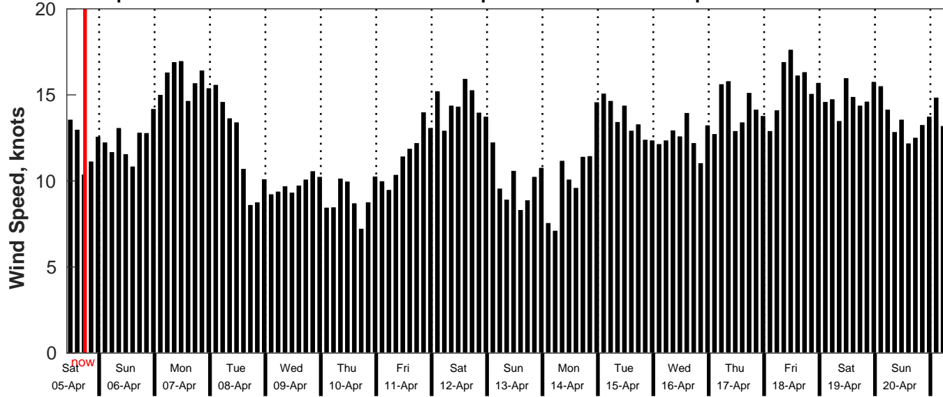
GFS Wind Speed Forecast for NDBC 52211 from 04-Apr-2025 10:00:00 to 20-Apr-2025 10:00:00
