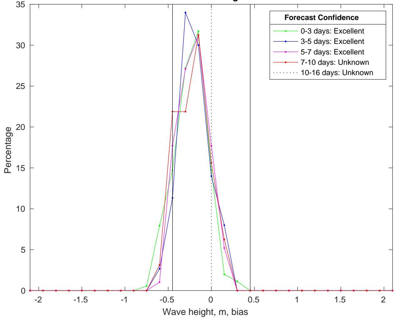
NDBC 52212 vs GFSWaves Bias Histogram: 18-Jan-2025
