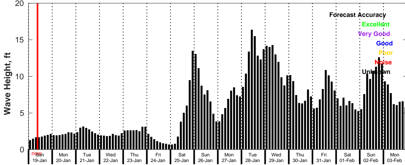
GFS Wave Forecast for NDBC 62305 from 18-Jan-2025 00:00:00 to 03-Feb-2025 00:00:00
